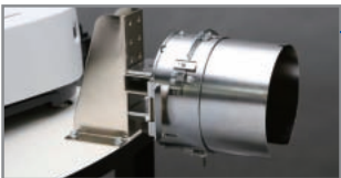
Tool attachments such as cap frames and cylindrical frames
